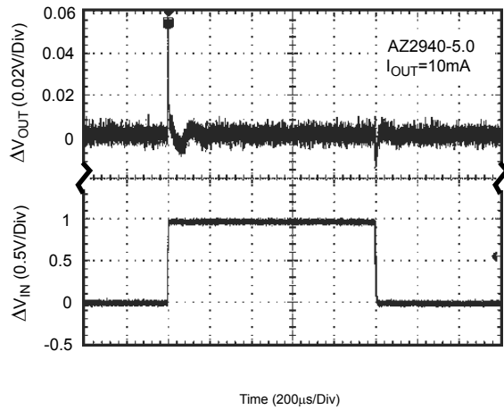
Figure 19. Line Transient
