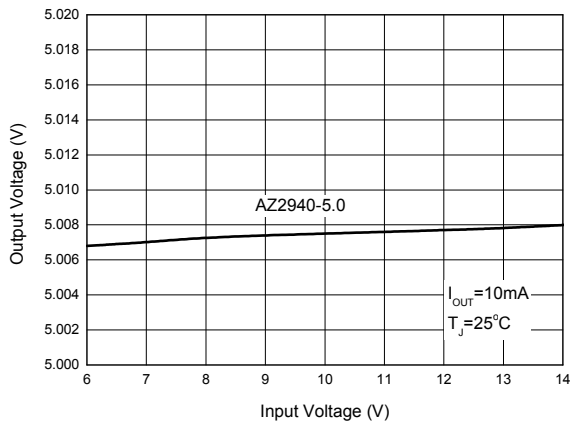
Figure 4. Line Regulation
