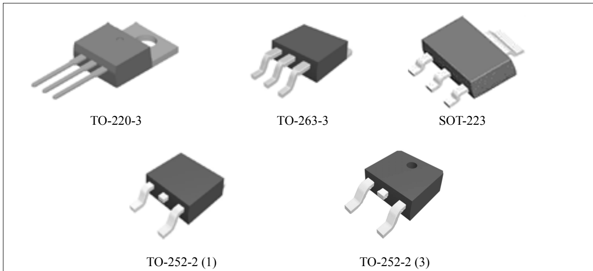
Figure 1. Package Types of AZ2940
