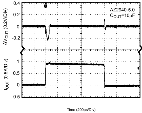
Figure 17. Load Transient
